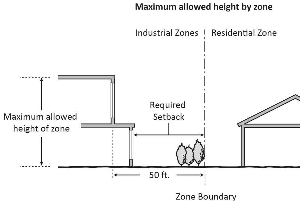
Figure 17.06.030-1: Transitional Height Standards
