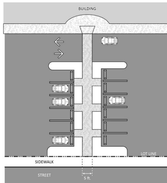
Figure 17.16.070-3: Alternate Parking Area Designs
