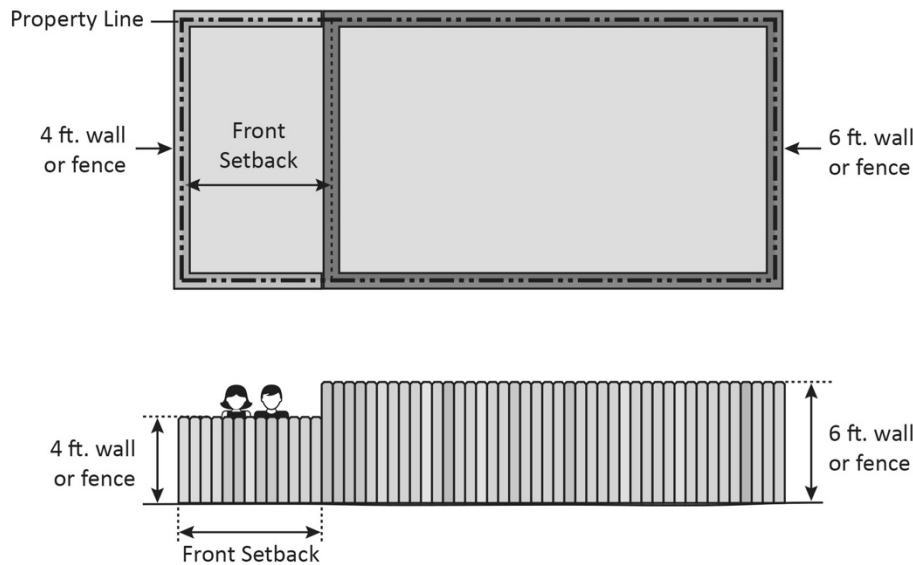
Figure 17.13.070-1 Measuring Front Setback.
