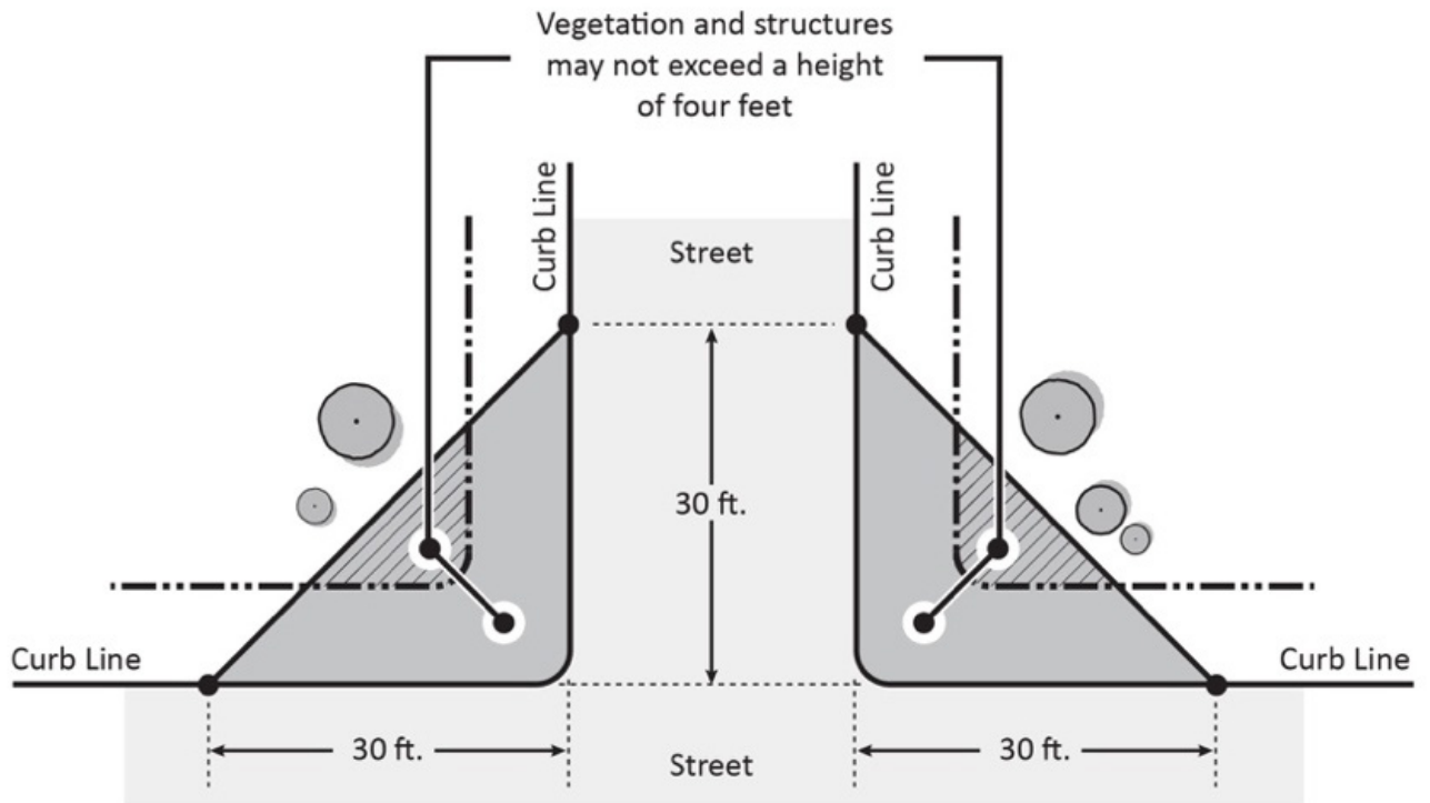
Figure 17.13.170-1 Visibility at Intersections.
