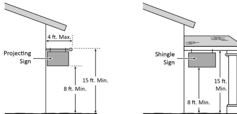
Figure 17.19.090-2 Projecting and Shing.
