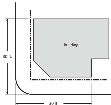
Figure 17.04.040-3 Corner Lot Setback.
