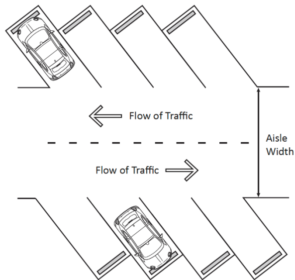
Figure 17.16.070-2: Aisle Dimensions
