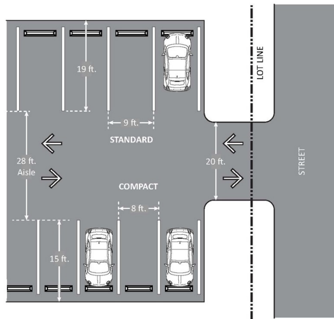
Figure 17.16.070-1 Parking Space Dimension.
