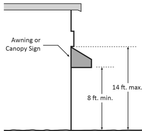
Figure 17.19.090-1 Awning and Canopy Signs.
